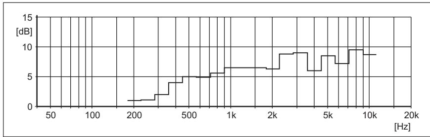
Directivity index
